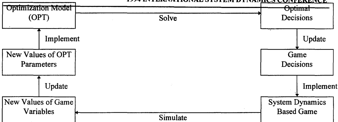
Figure 1: Evaluating Optimization Models
