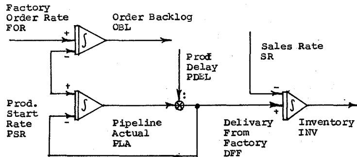
Fig. 3 Analogue Representation of the Reduced Basic System
