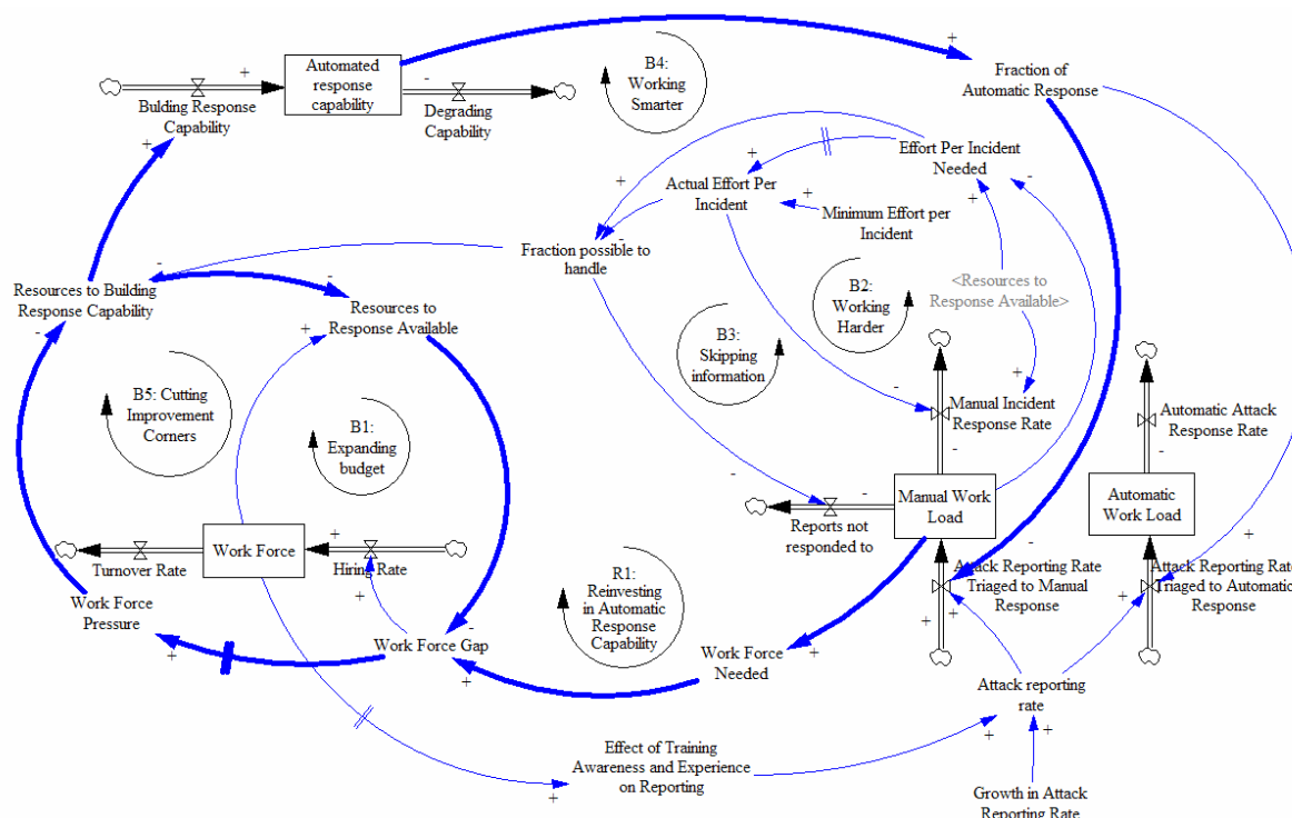
Figure 11: Work force pressure can generate unintended side-effects
