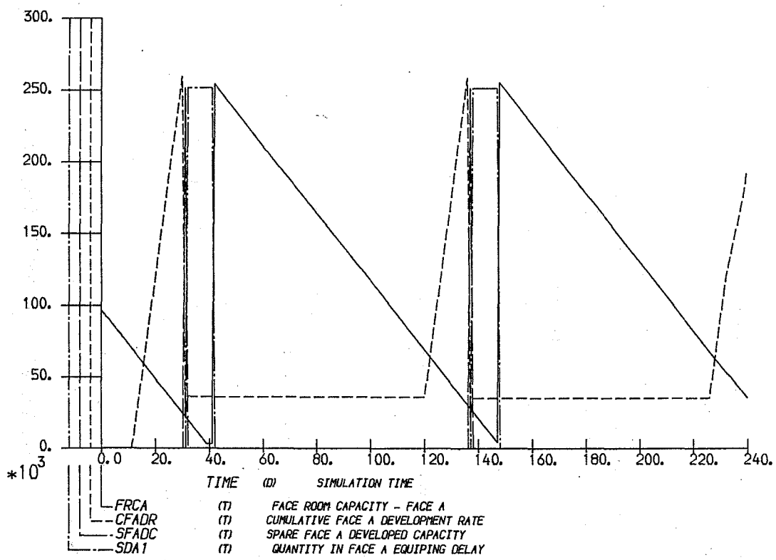
FIGURE 8. MODEL GENERATED FACE DYNAMICS
