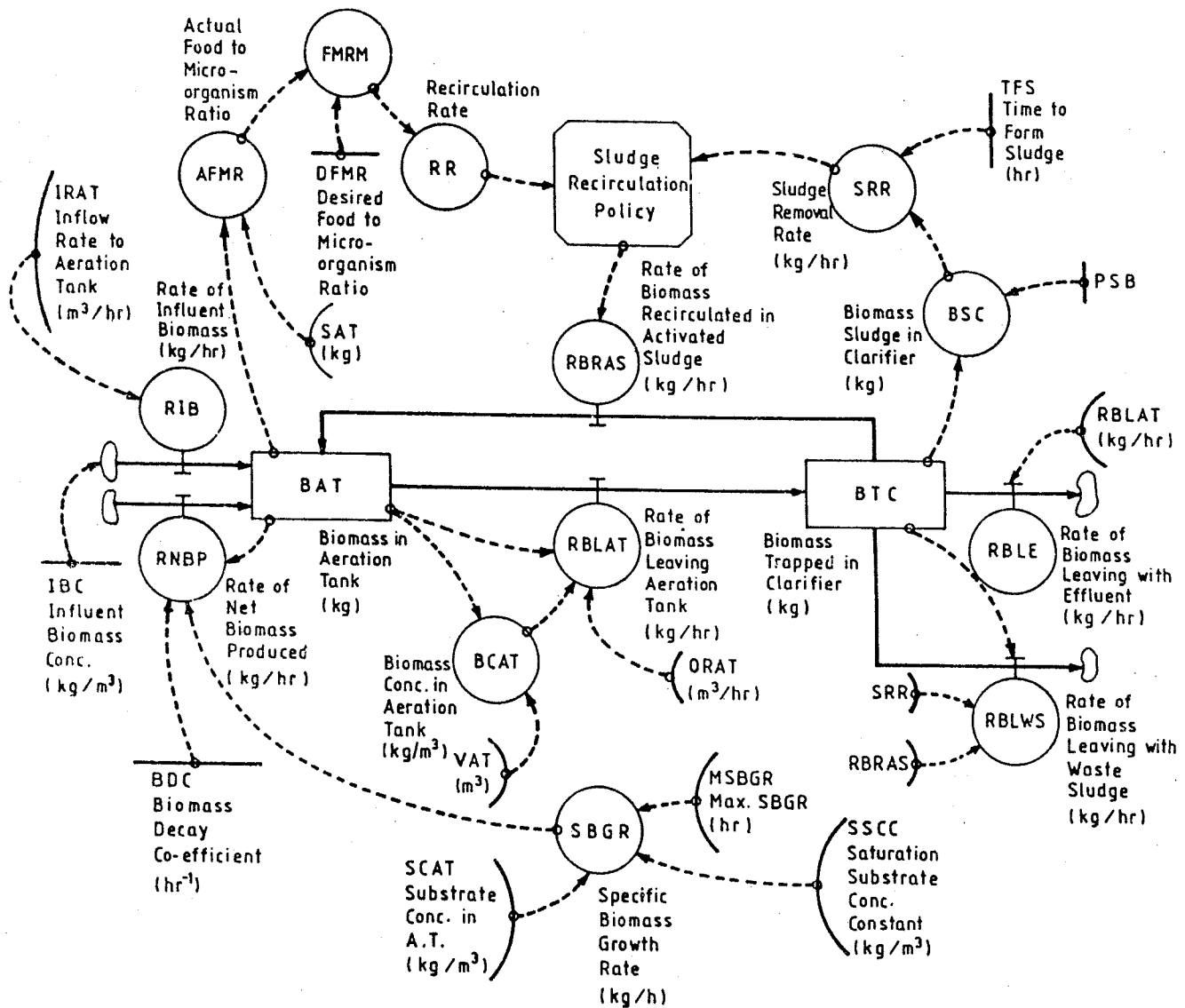
Figure 3 Flow Diagram for Biomass with ASP System.
