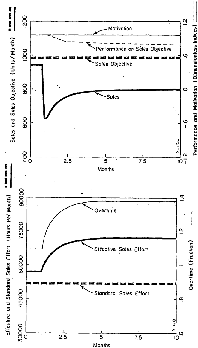
Figure 7. Salesman Overtime Adjustment Loop 1 in Isolation
