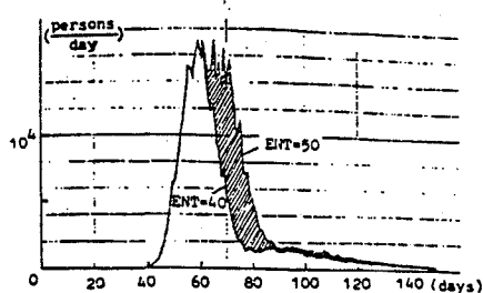
Fig. 9 A Comparison between Two Simulated Spread Curves with Different Prohibition Times
