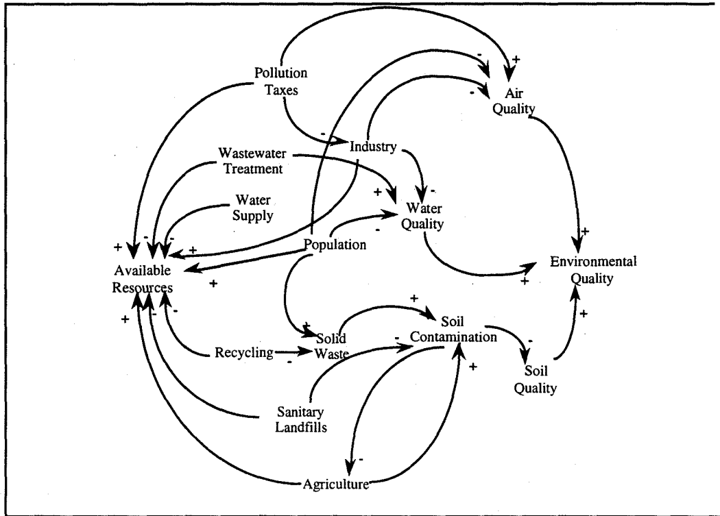
Figure 1 - Causal diagram
