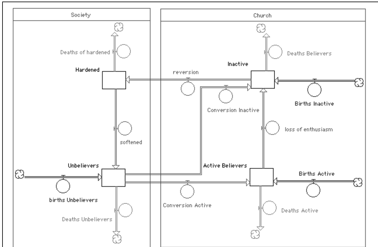
Fig. 15. Outline of limited enthusiasm conversion model with births, deaths and reversion. Conversion details are suppressed but are similar to figure 12.
