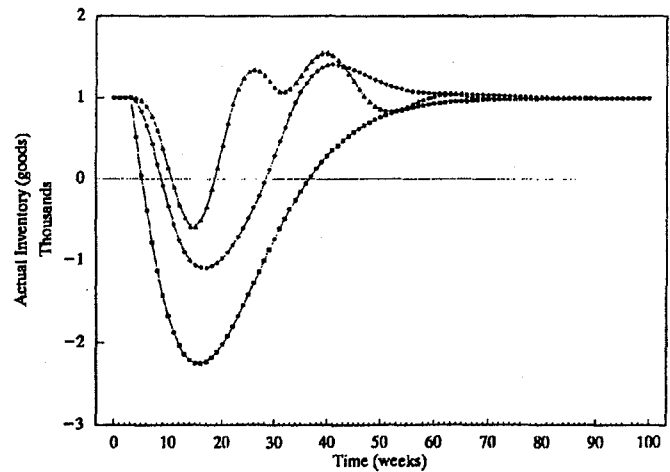
Figure 6. Dynamics of a Constrained Supply Chain with Improved Parameter Settings
