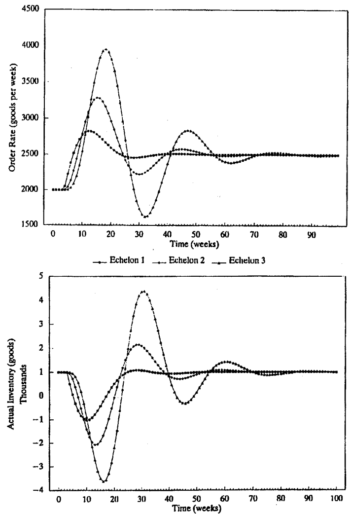
Figure 4. Dynamics of an Unconstrained Supply Chain (Simulation Number 1) for a Step Input
