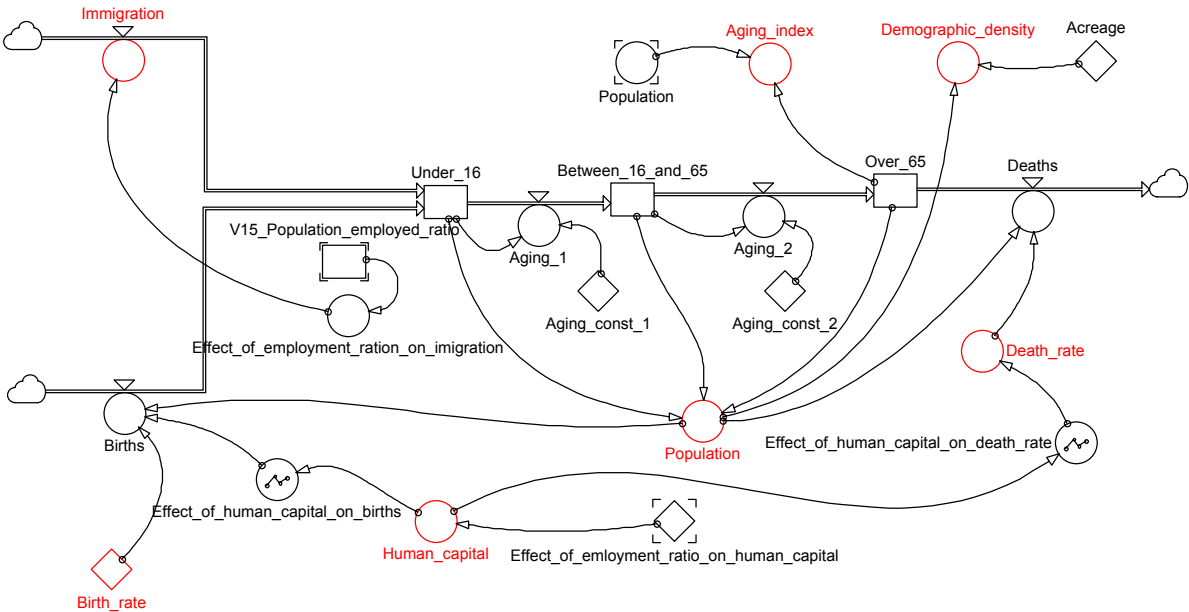
Figure 2: Population sub-model
