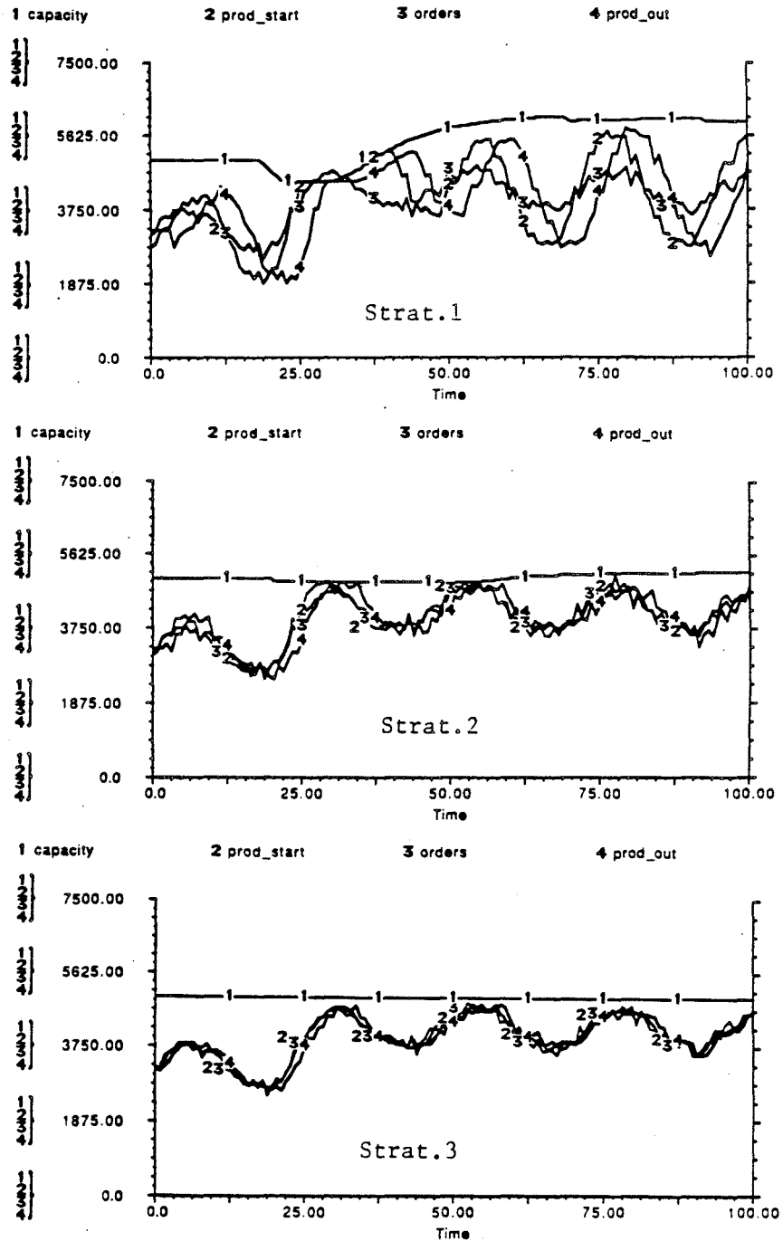
Fig.4: Orders, materials flow and capacity
