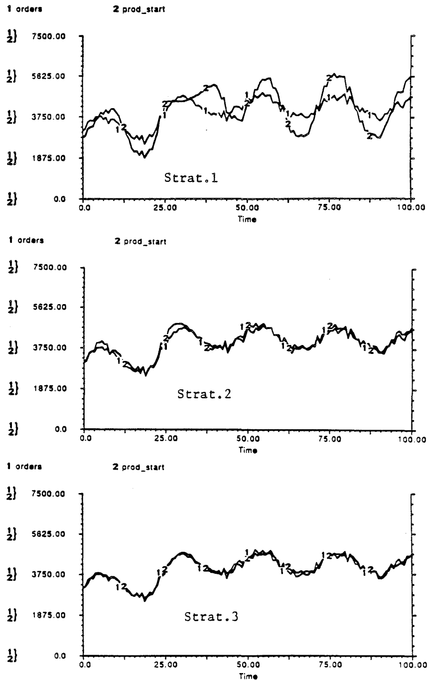
Fig.6: Orders and production starts response of system
