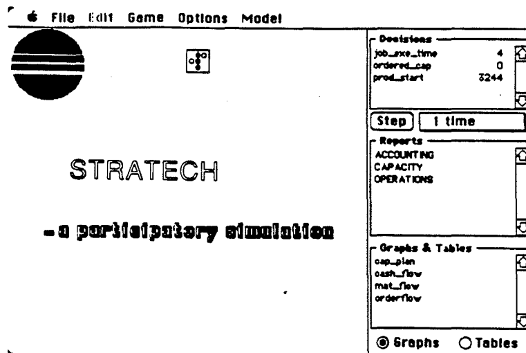
Fig.9: Microworld spreadsheet
